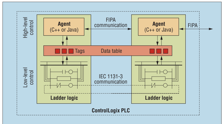
Figure 4. A real-time control agent architecture for the ControlLogix programmable logic controller. (FIPA stands for the Foundation for Intelligent Physical Agents; IEC stands for the International Electrotechnical Commission.)
